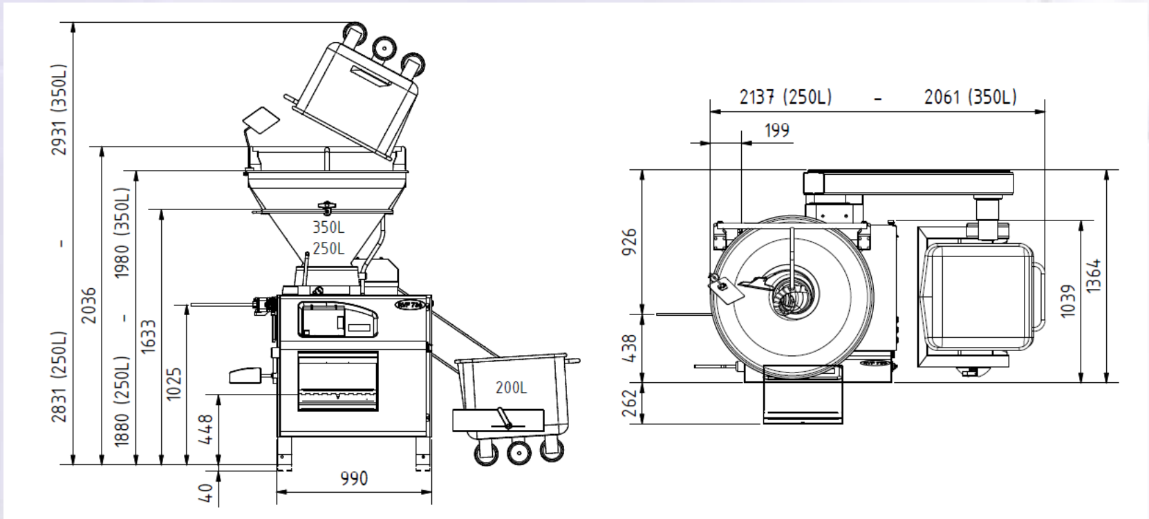
■ Dimensioned drawing RVF 700 with 250 & 350 litre hopper
